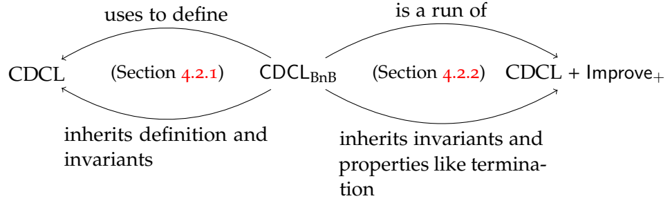
Figure 4.1: \text{CDCL}_{\text{BnB}} , CDCL, and Incremental CDCL
