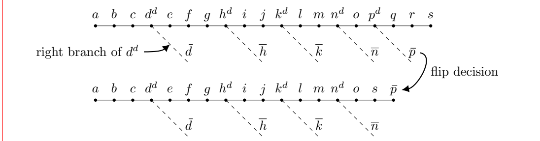
Figure 2: Trail after backtracking chronologically in \text{Back}\{\text{True}, \text{False}\} . The trail itself together with the dashed lines represents the pending search space, i.e., the assignments not yet tested.
