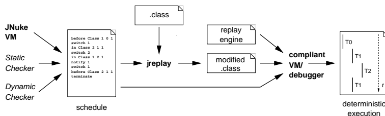
Fig. 4. Overview of jreplay
